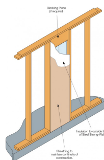
Steel Strong-Wall installation example.
