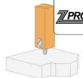
PBWS post installation using 4 x CSA connector screws.
