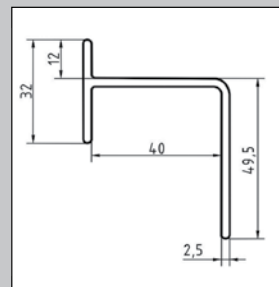
Drawing of top profile
