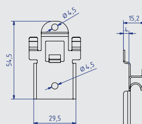
Façadeclip Rhombus
