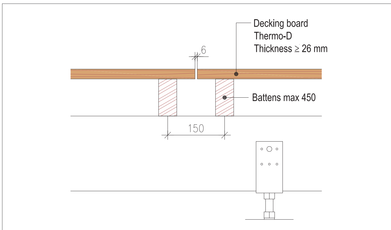
Figure 49. Decking board joint.
