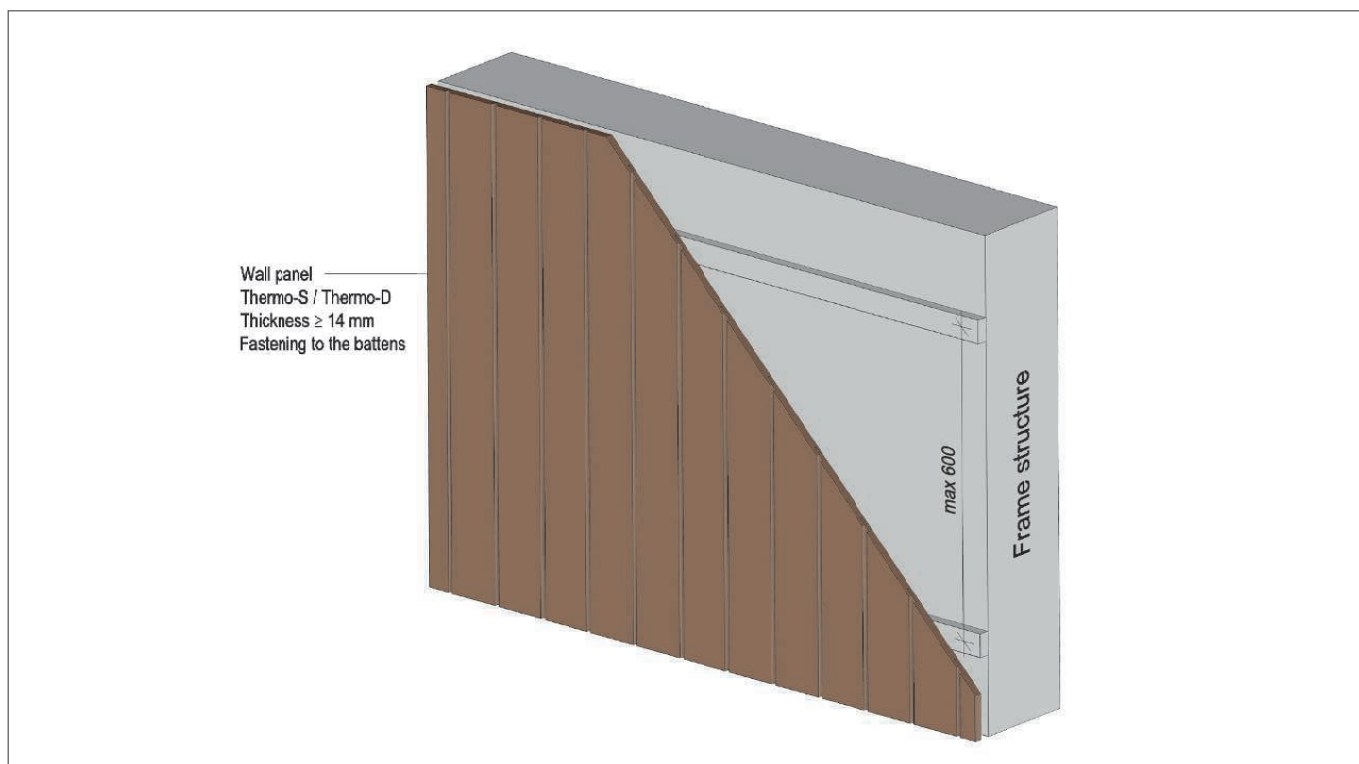
Figure 39. An example of interior wall cladding.
