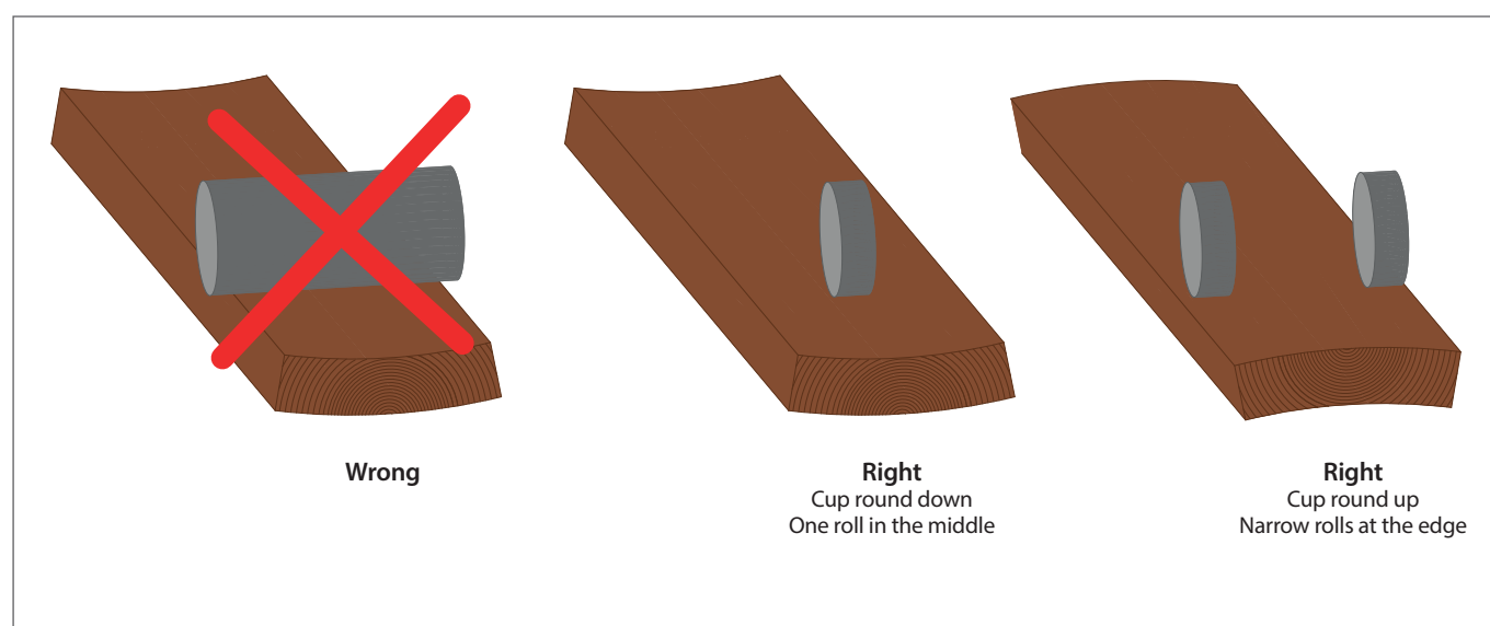
Figure 32. Narrow plane infeed rollers must be used with ThermoWood® products.
