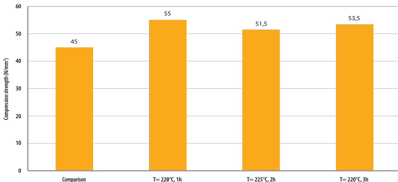
Figure 25. Compression strength parallel to the grain of thermally modified spruce (average density 420 kg/m³) (source: VTT).
