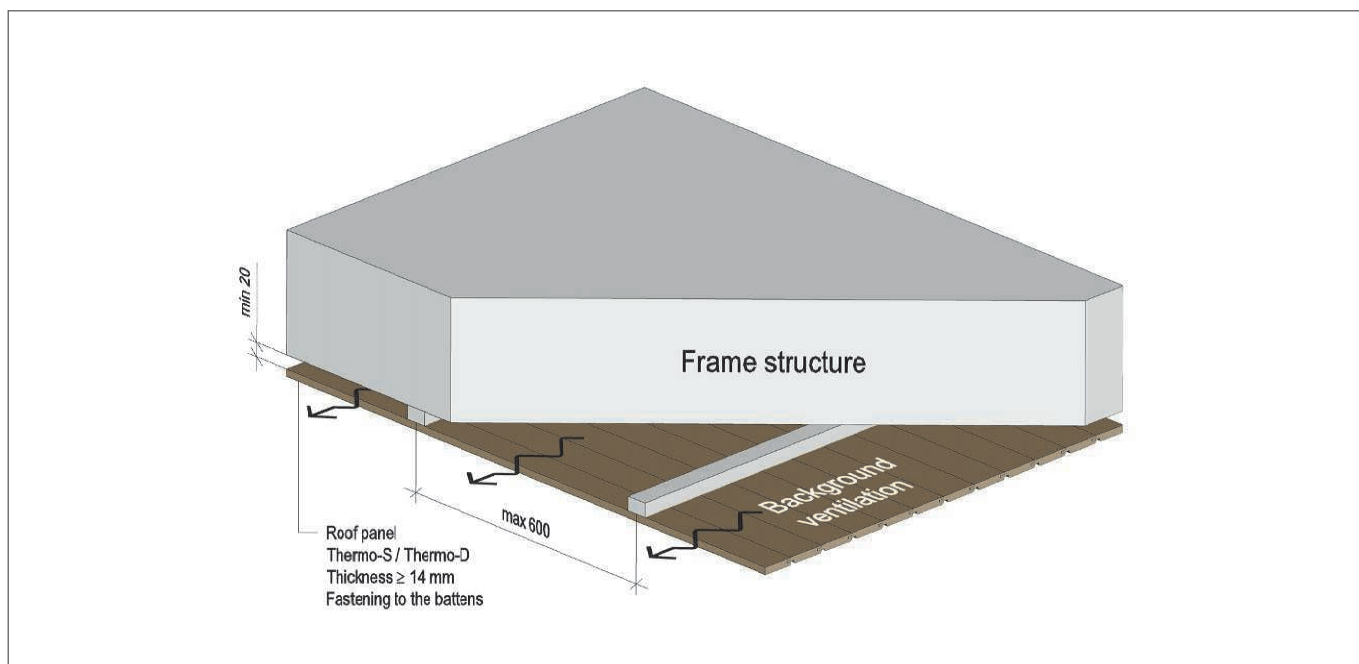
Figure 41. An example of ceiling cladding for a sauna.
