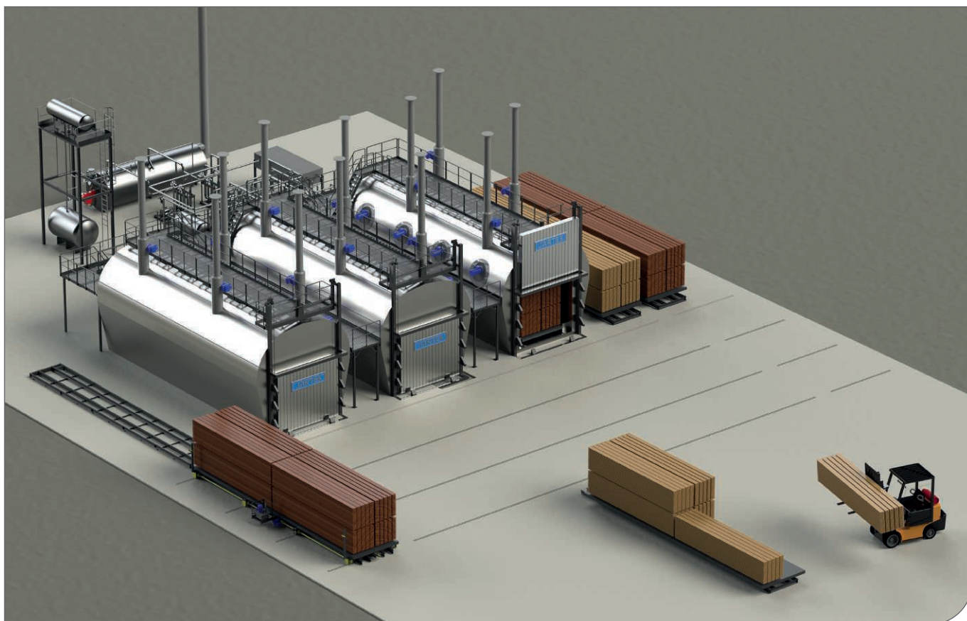
Figure 7. ThermoWood® plant.
