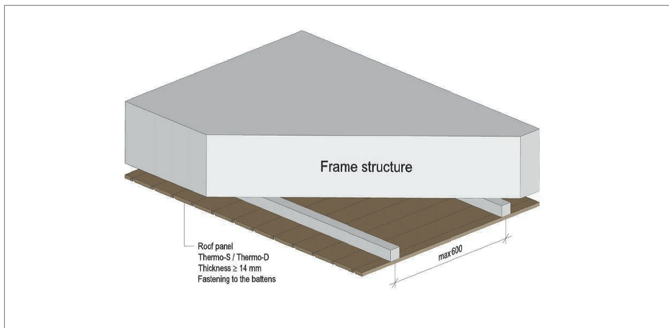
Figure 37. An example of ceiling cladding in a dry space.
