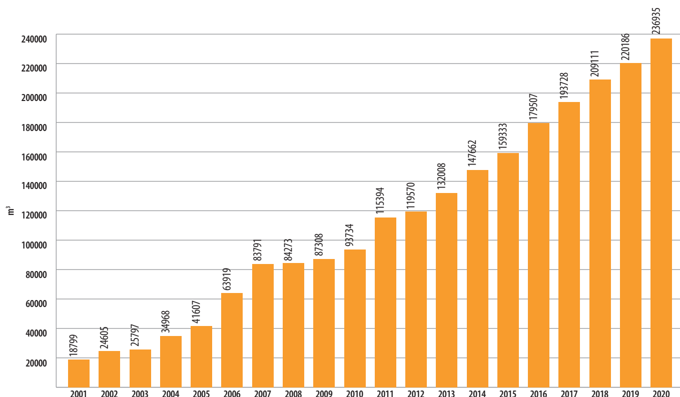
Figure 1. Changes in ThermoWood® production between 2001 and 2020.
