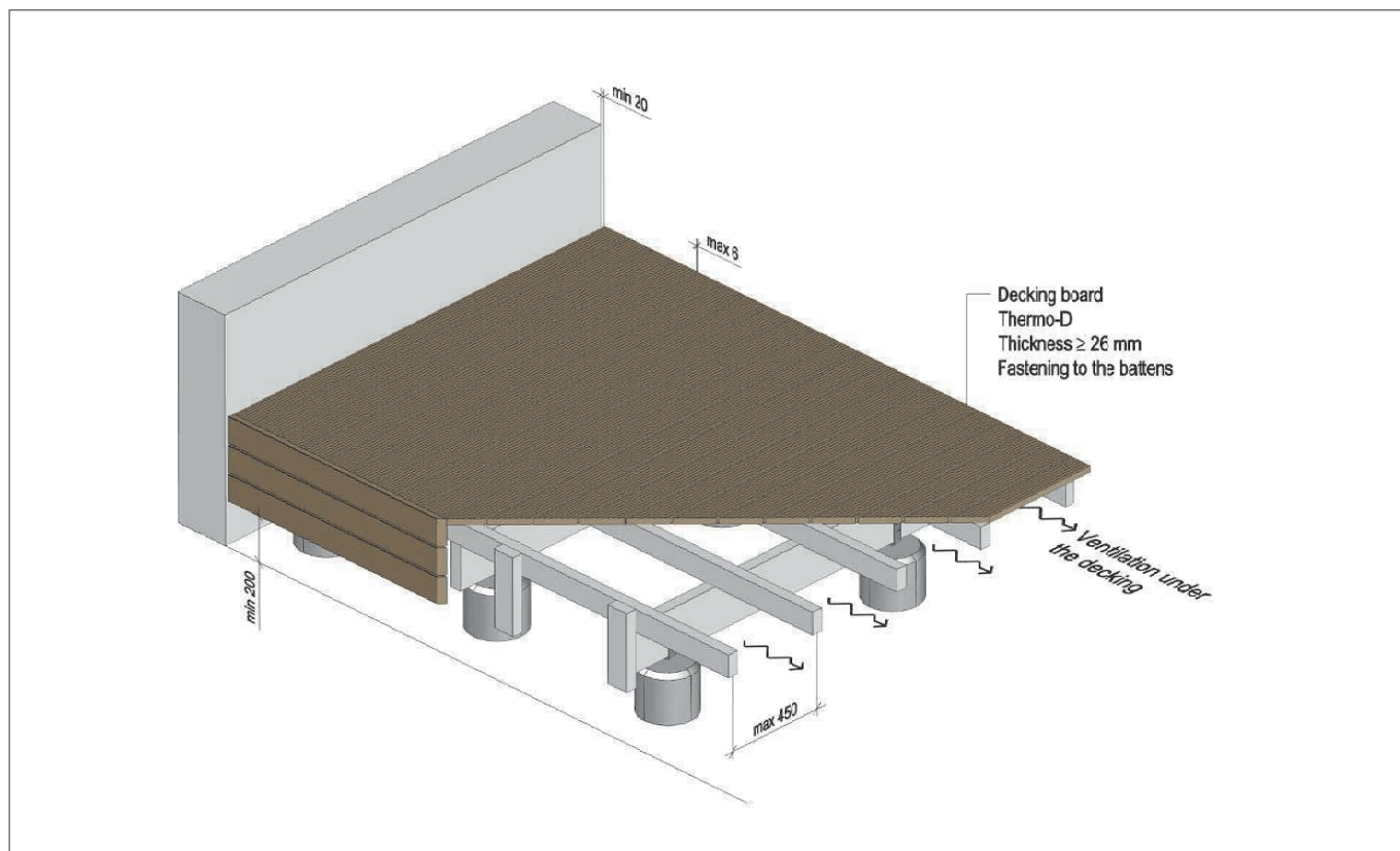
Figure 48. An example of patio structures.
