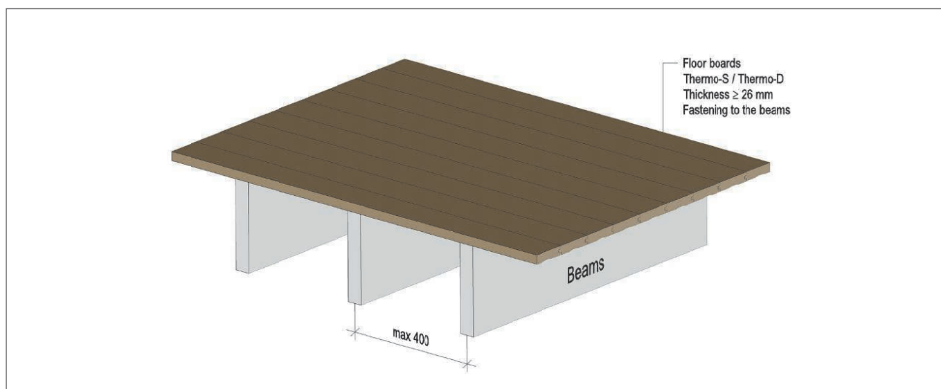
Figure 35. An example of flooring.
