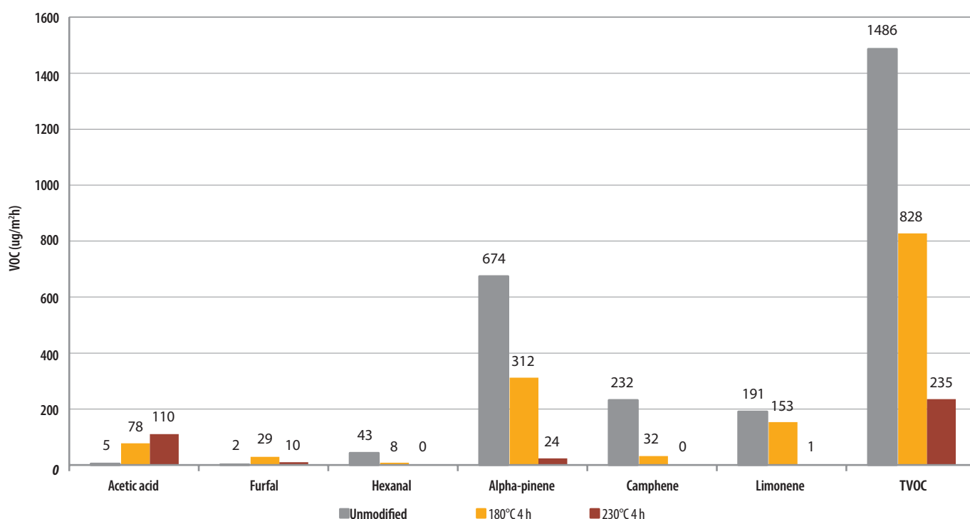
Figure 31. Volatile organic compounds emitted by pine samples after two months (source: VTT).
