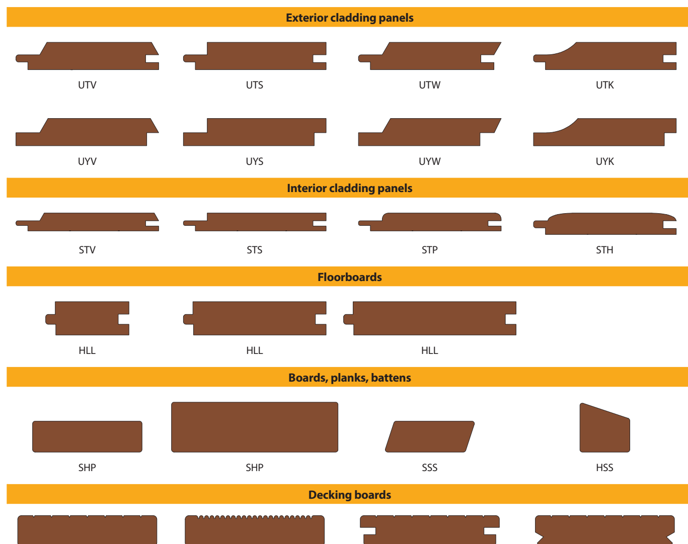
Figure 14. Examples of ThermoWood® profile products.
